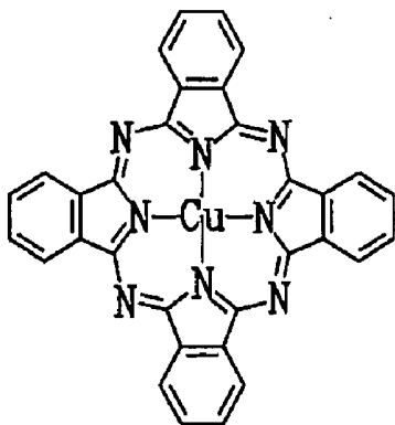
CuPC
